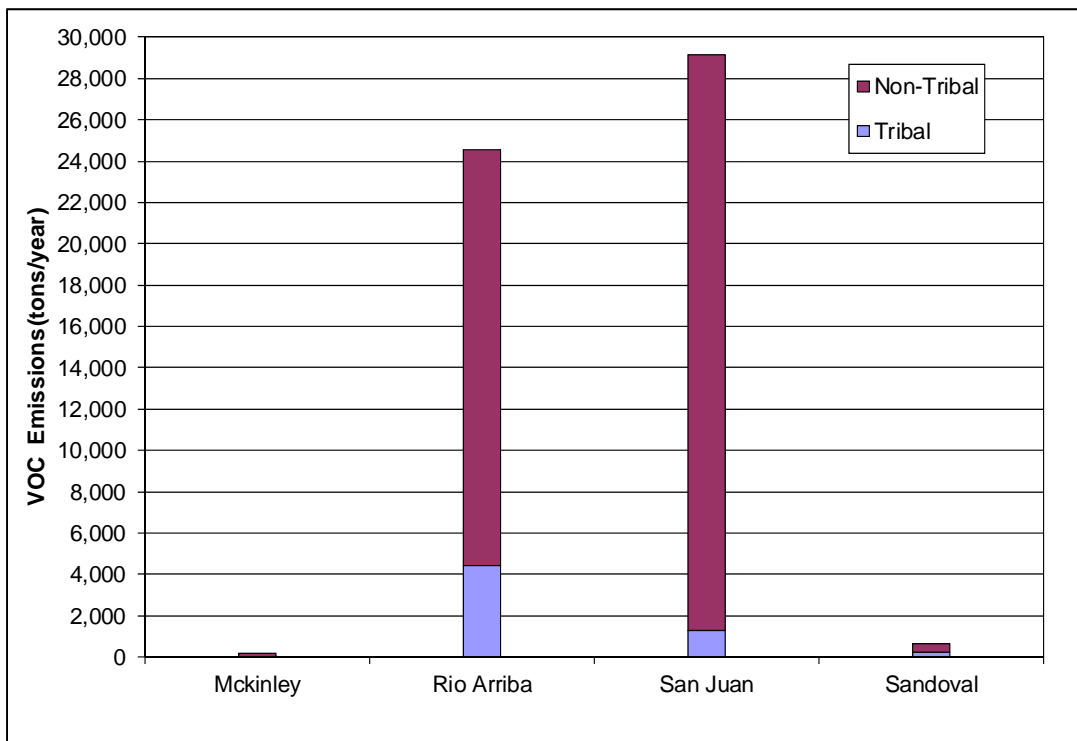
Figure 8. 2008 South San Juan Basin projected VOC emissions by tribal vs. non-tribal land for each county.
