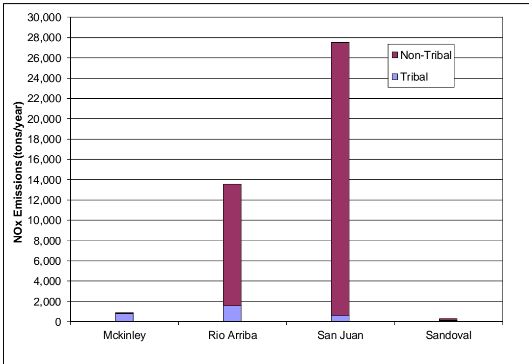
Figure 7. 2008 South San Juan Basin projected NOx emissions by tribal vs. non-tribal land for each county.
