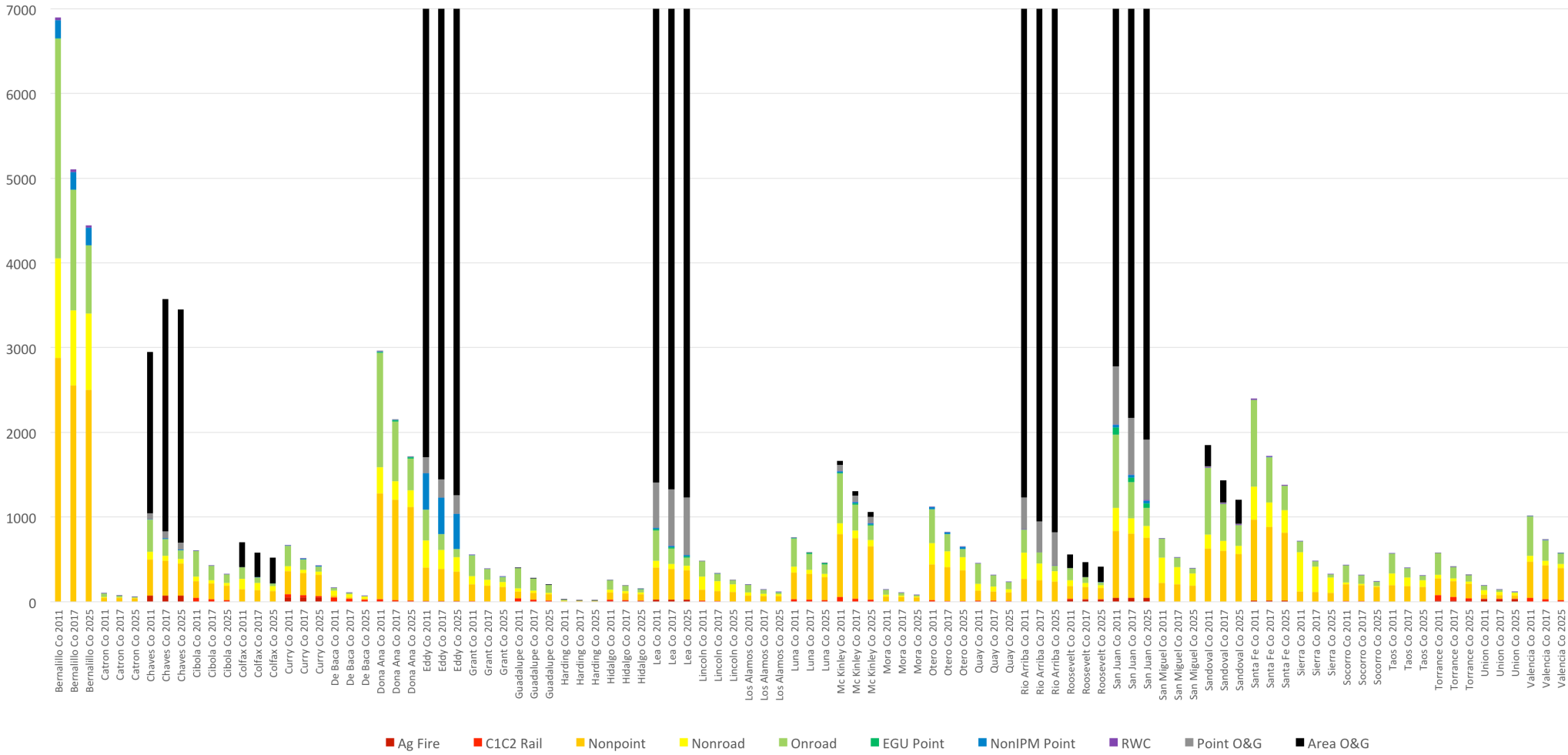
US EPA NEI2011v6.2 May - Sept New Mexico County VOC_INV Emissions: 2011, 2017, 2025
