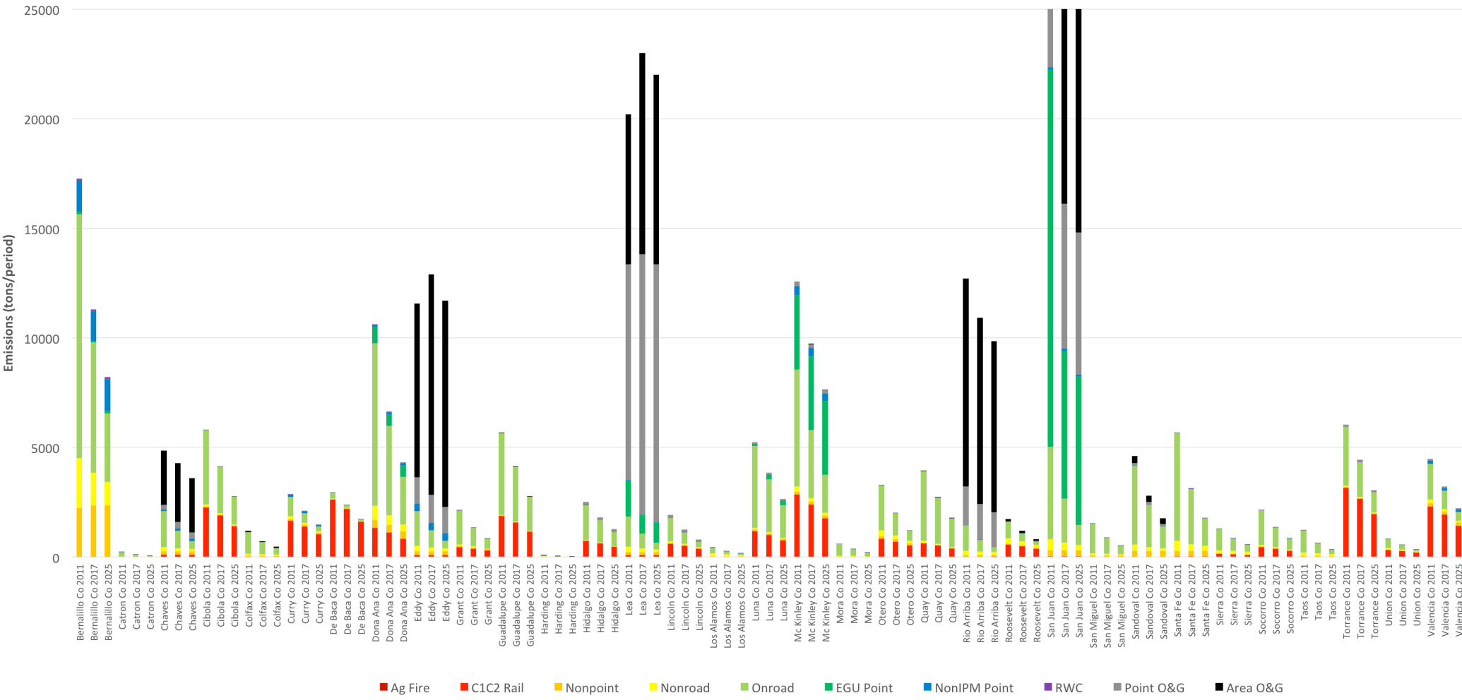
US EPA NEI2011v6.2 Annual New Mexico County NOx Emissions: 2011, 2017, 2025
