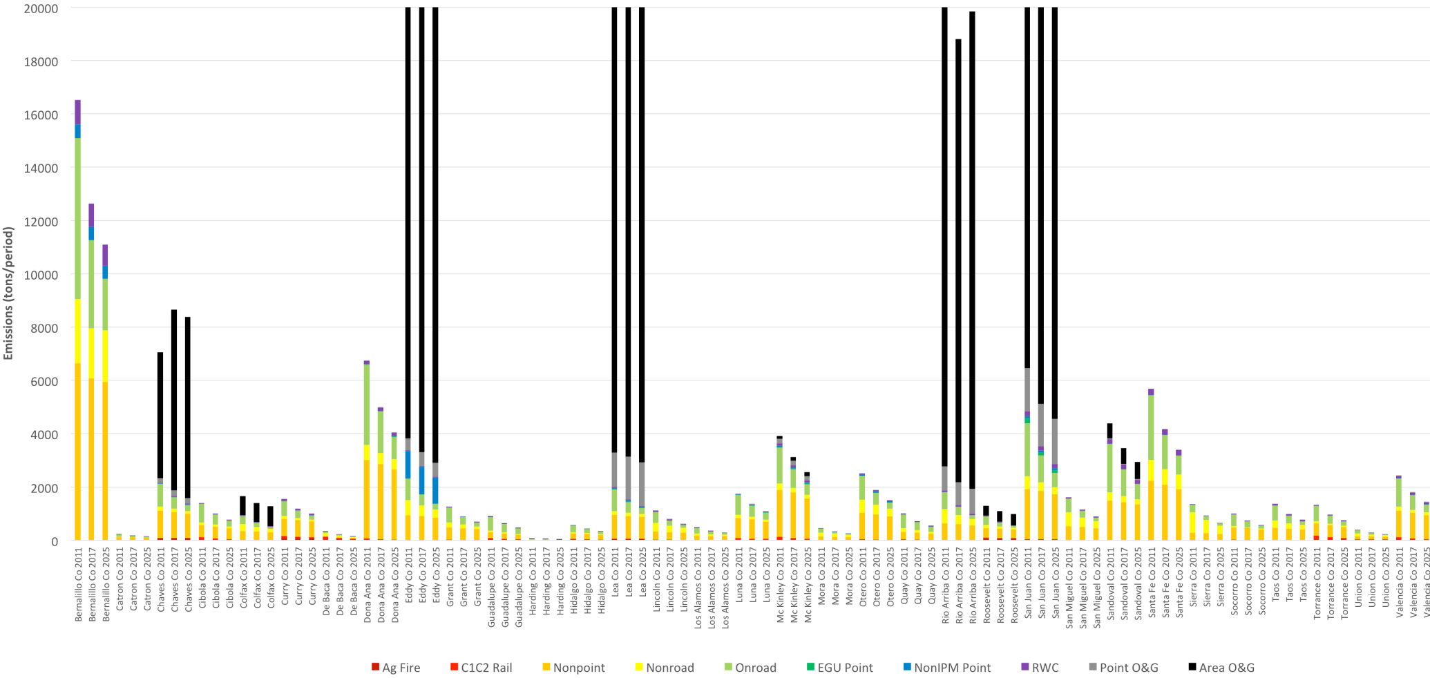
US EPA NEI2011v6.2 Annual New Mexico County VOC_INV Emissions: 2011, 2017, 2025
